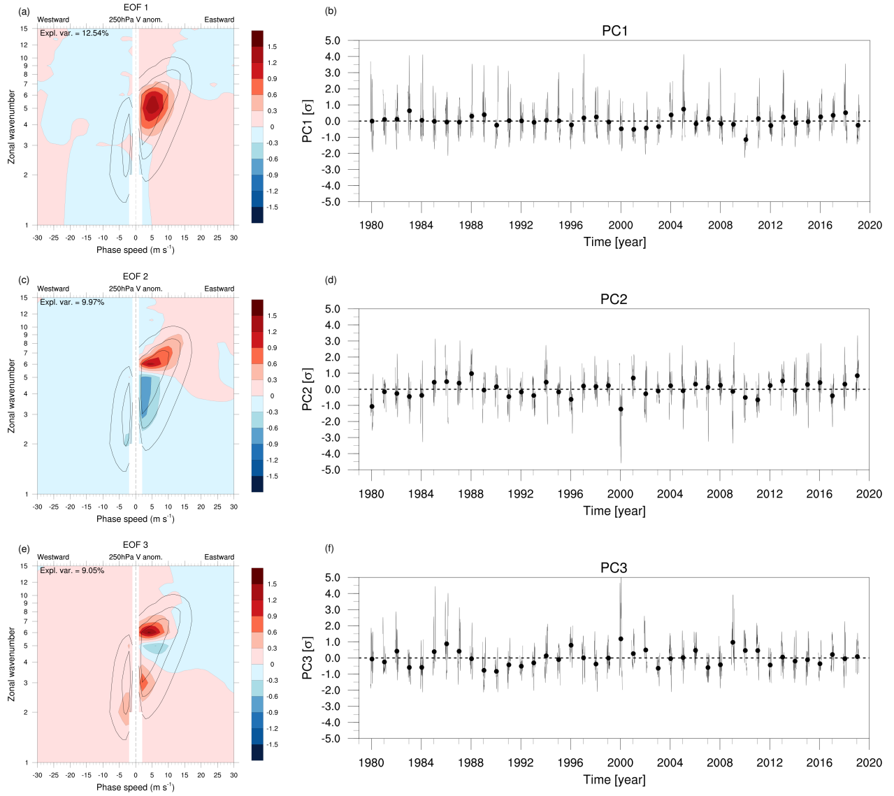
Figure 2. (a,c,e) Loadings of the first three EOFs of daily spectral anomaly during DJF (shaded, arbitrary units). The climatological spectral power is overlaid (black contours as in Fig. 1, only the 0.2, 0.4 and 0.6 \text{m s}^{-1} \Delta c^{-1} levels). (b,d,f) Principal components associated with each EOF (standardized).
